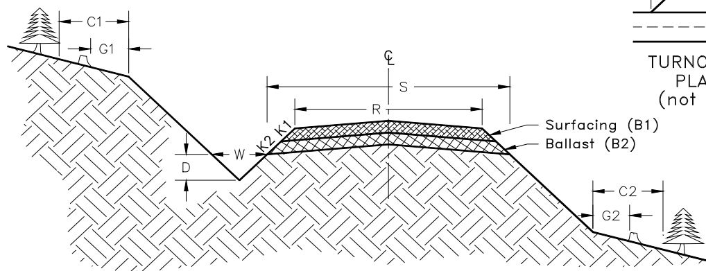
ROAD CROSS-SECTION (not to scale)
