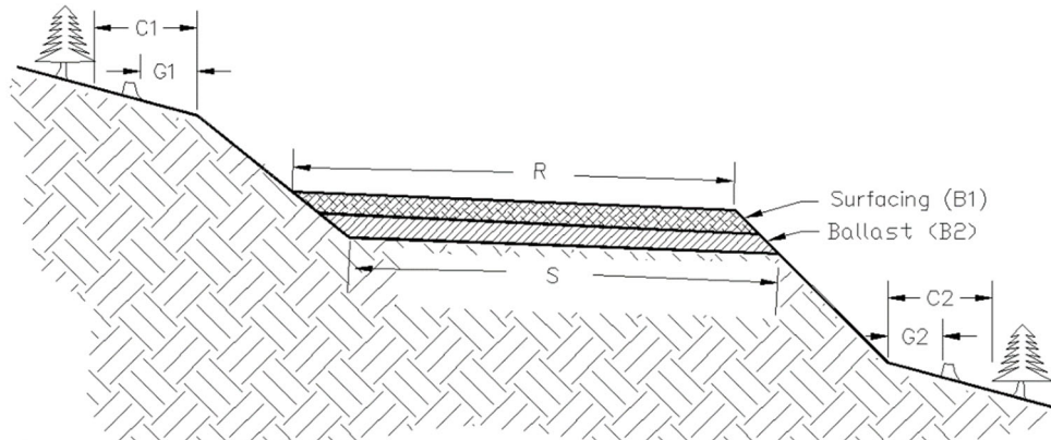
OUTSLOPED ROAD CROSS-SECTION (not to scale)
