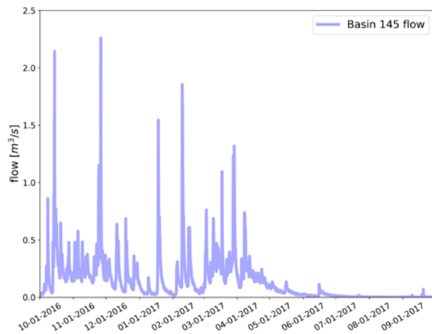
Figure 8. Hydrograph from one of the managed watersheds showing data from one water year
