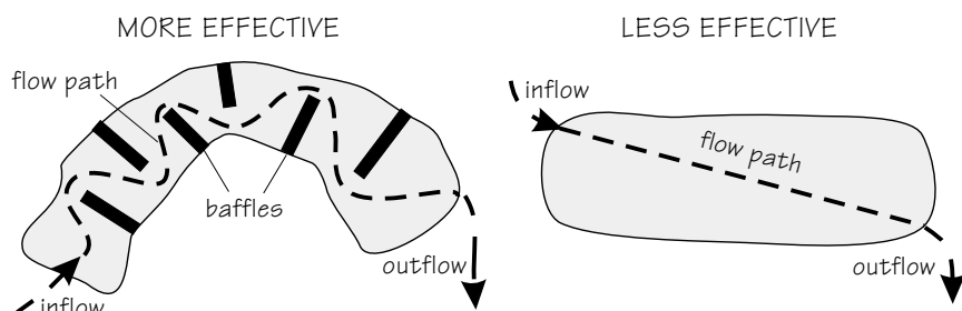
Figure 2.30. Details of detention pond design. The pond on the left, which maximizes the length of the flow path, is preferable to the pond on the right, which does not keep water in the pond long enough for optimum settling.
