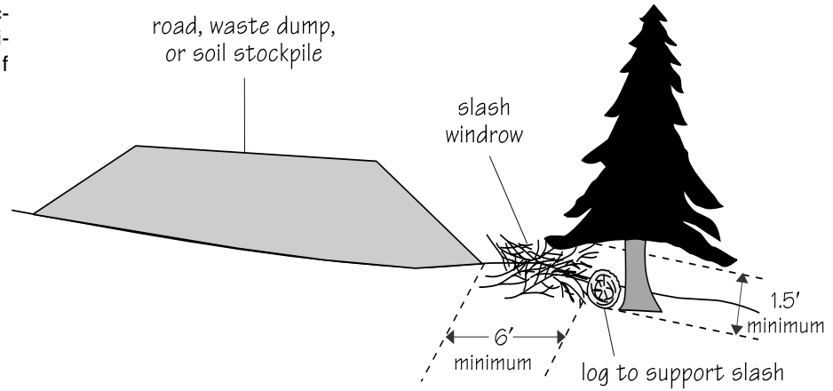
Figure 2.13. Details of construction of a slash windrow filter. (Modified from Idaho Department of Lands, 1992.)
