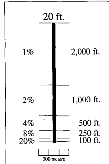
Figure 16. Example of a gradient template used with a USGS 7.5 minute 1:24,000 scale topographic map and having 20 ft. contour intervals.
