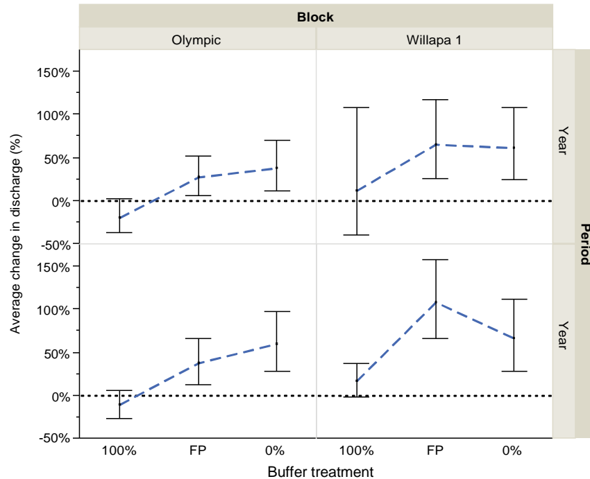
Figure 8-6. Relative change in mean discharge (%ΔQ) with 95% confidence intervals (CI) for the first (Year 1) and second (Year 2) years post-harvest, by treatment and block.
