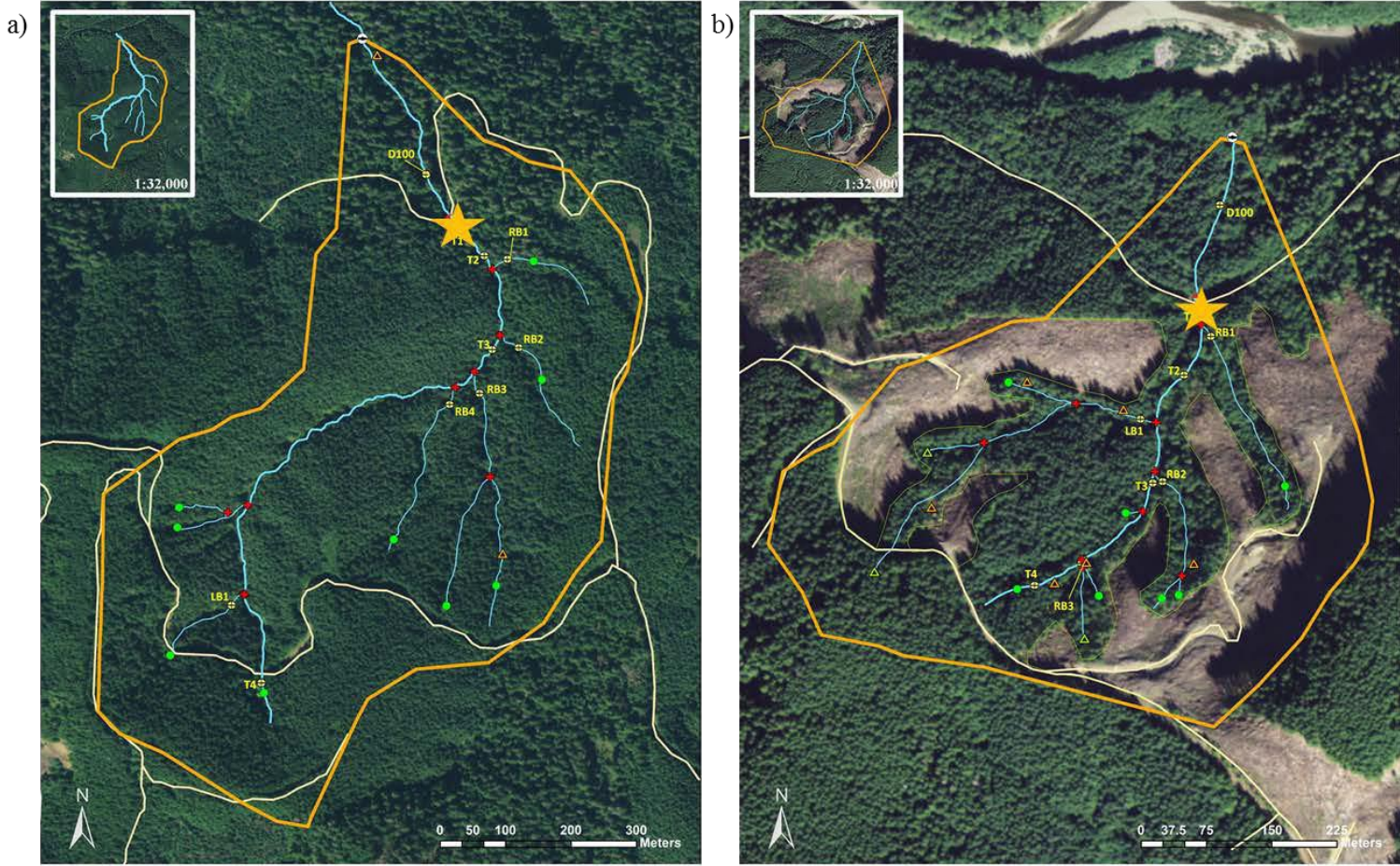
Figure 14-2. Location of the culvert and drift net installed in the Olympic Block (a) unharvested reference (OLYM-REF) and (b) 100% treatment (OLYM-100%).
