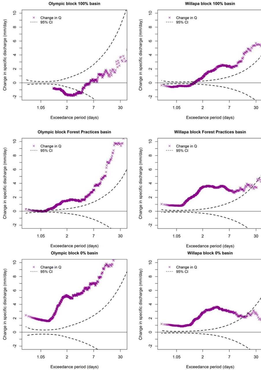
Figure 8-10. Absolute change in specific discharge as a function of the number of days that a discharge is exceeded. Confidence intervals (CI) become very large for events with an exceedance period of greater than 7 days so we restricted the analysis to recurrence intervals (RI) <30. In the 100% sites, discharge decreases for RIs <2 days and in most sites significant (i.e., beyond 95% CI) change occurs between the 2-day and 7-day RI.
