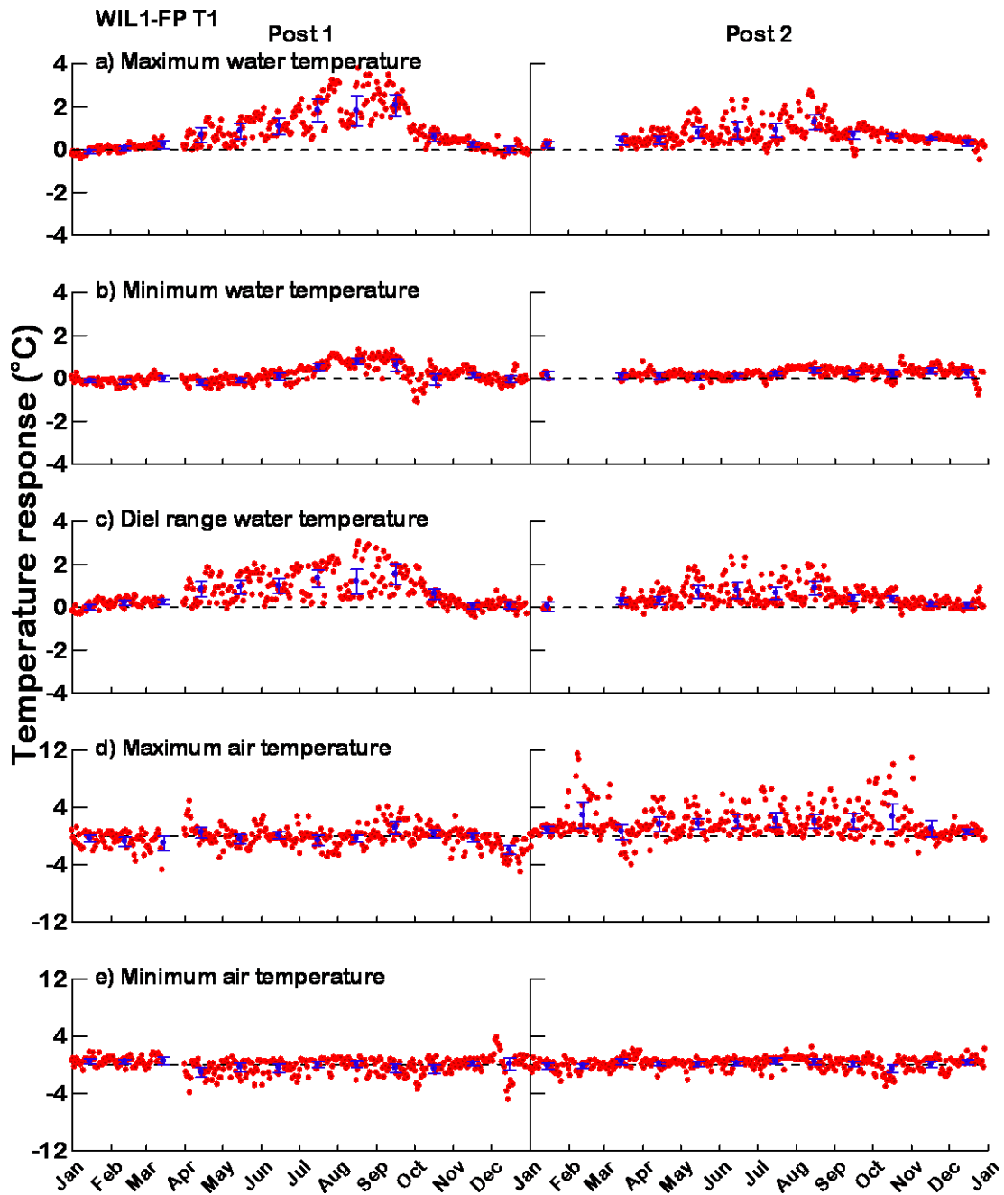
Appendix Figure 7-C-6. Water temperature and air temperature response at site WIL1-FP, location T1. Red dots are the daily temperature response (TR). Blue dots and error bars are the mean monthly temperature response (MMTR) with 95% confidence intervals (CI).
