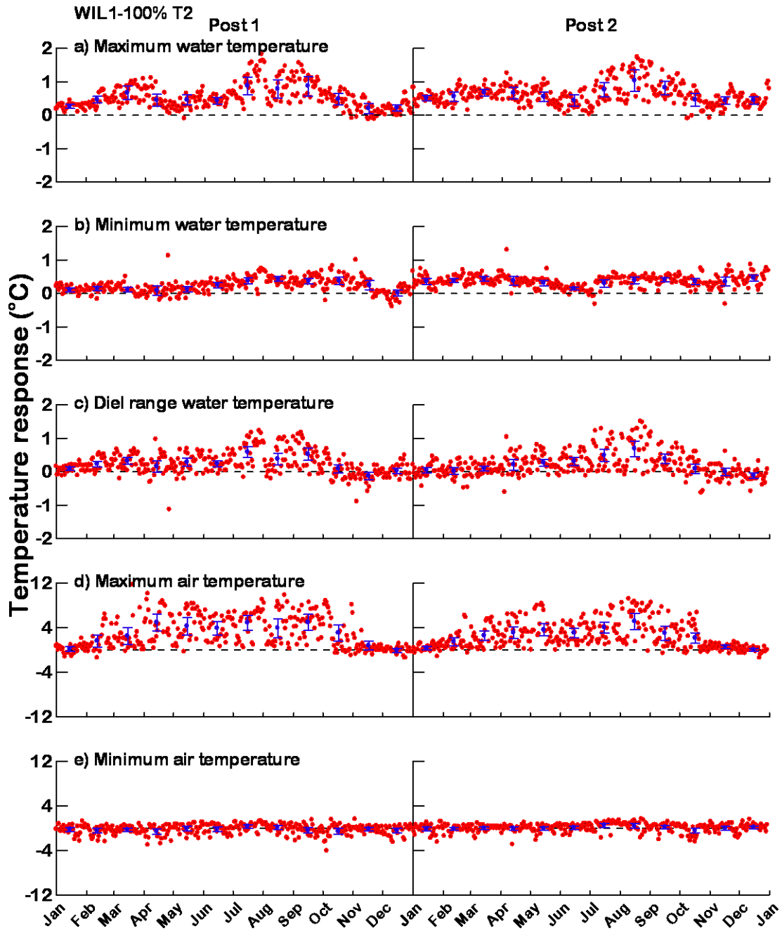
Appendix Figure 7-C-2. Water temperature and air temperature response at site WIL1-100%, location T2. Red dots are the daily temperature response (TR). Blue dots and error bars are the mean monthly temperature response (MMTR) with 95% confidence intervals (CI).
