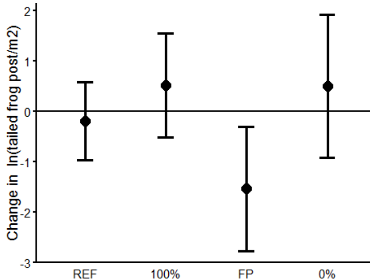
Figure 15-8. The within-treatment change for the natural log (ln) of post-metamorphic Coastal Tailed Frog density (animals/m 2 ), i.e., [ln(post) – ln(pre)], and 95% confidence interval (CI) estimated with rubble-rouse sampling in the lower Np reach for each of four treatments.
