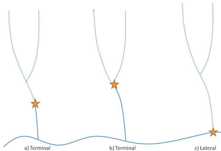
Figure 3-1. Types of F/N breaks: terminal break where the last fish occurs within a Type F Water (a), terminal break where the last fish occurs below the confluence of two Type N Waters (b), and lateral break where a Type N Water laterally intersects a Type F Water (c). Solid blue lines are Type F Waters, dashed blue lines are Type N Waters, and stars indicate F/N breaks.
