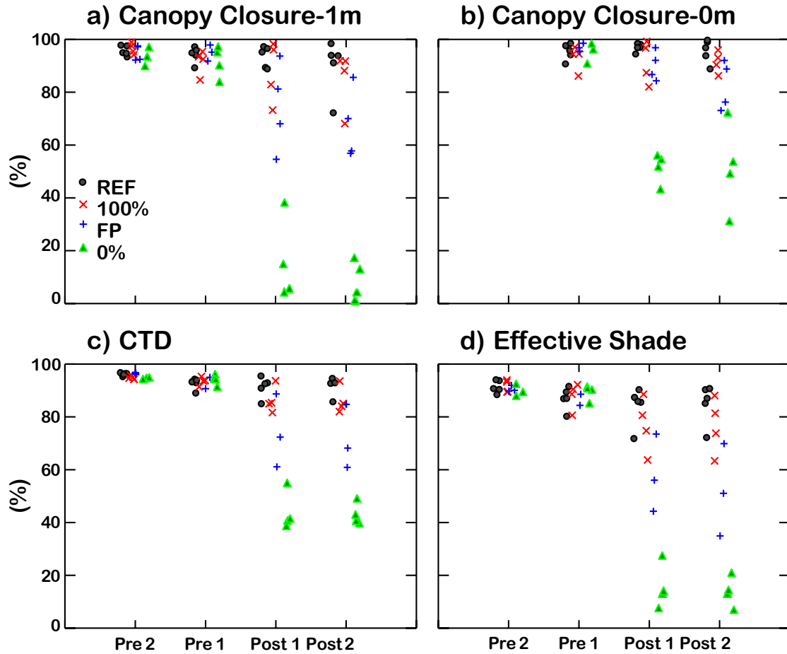
Figure 7-2. Mean site values for each stream cover metric. We did not calculate CTD (Canopy and topographic density) and effective shade for WIL1-0% in 2008. We did not measure canopy closure-0m until 2008 (Pre 1 year above).
