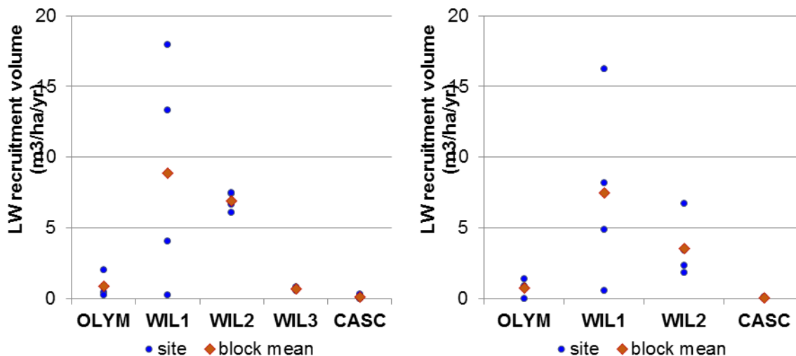
Figure 6-5. Site mean LW recruitment rates for RMZs (left panel) and PIPs (right panel) by block for the pre-harvest period.
