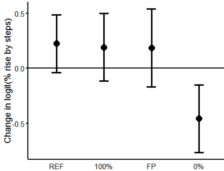
Figure 11-20. The within-treatment change and 95% confidence intervals (CI) for the logit-transformed channel rise (%) attributed to steps, i.e., [logit(post) – logit(pre)].
