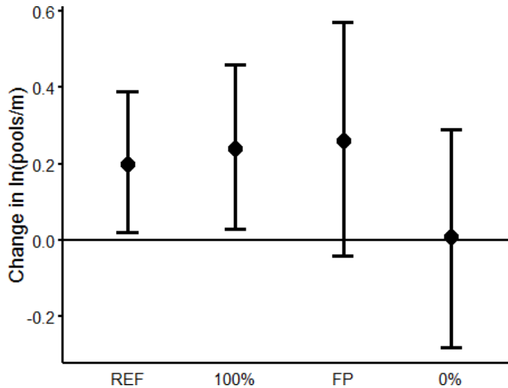
Figure 11-13. The within-treatment change and 95% confidence interval (CI) for the natural log (ln) of pool density (number/m), i.e., [ln(post) – ln(pre)].
