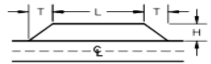
TURNOUT DETAIL PLAN VIEW (not to scale)
