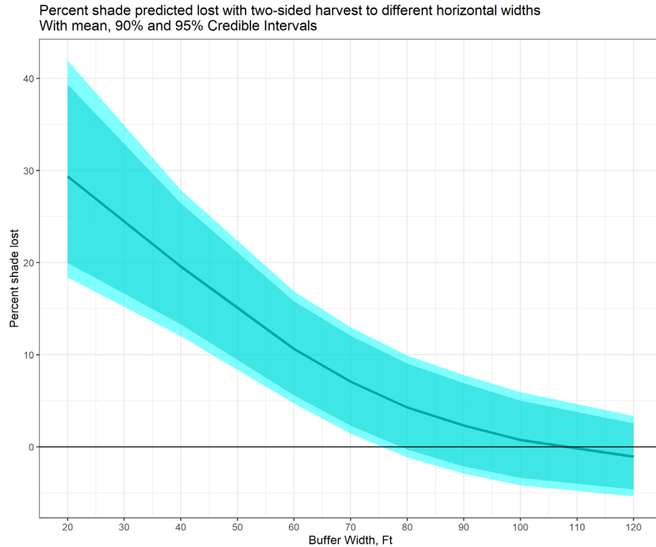
Figure 2: Predicted relationship between two-sided buffer width and percent shade lost post-harvest. This prediction was based on the data and analysis approach of Groom et al. (2018).
