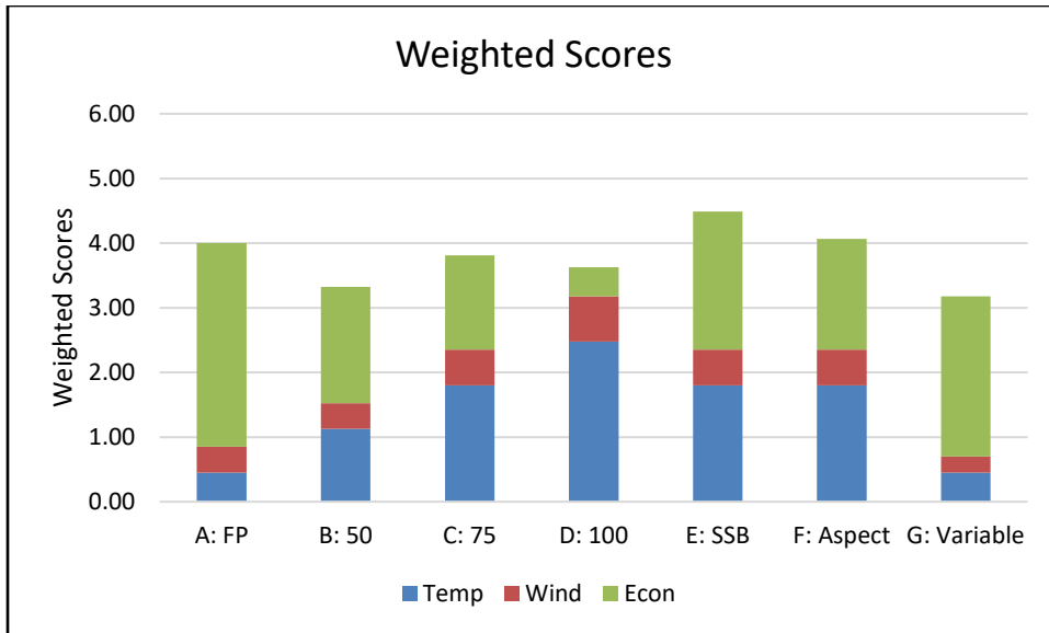
Figure A4: Performance of weighted score values for Alternatives A through G. SSB is an acronym for Site-Specific Buffer.
