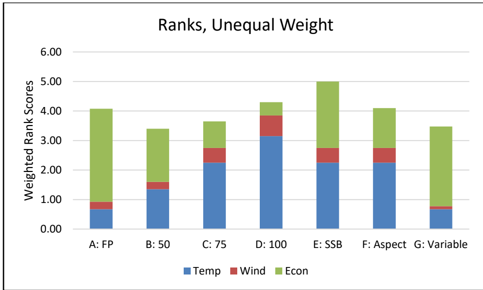
Figure A3: Performance of unequally weighted ranks for Alternatives A through G. SSB is an acronym for Site-Specific Buffer.
