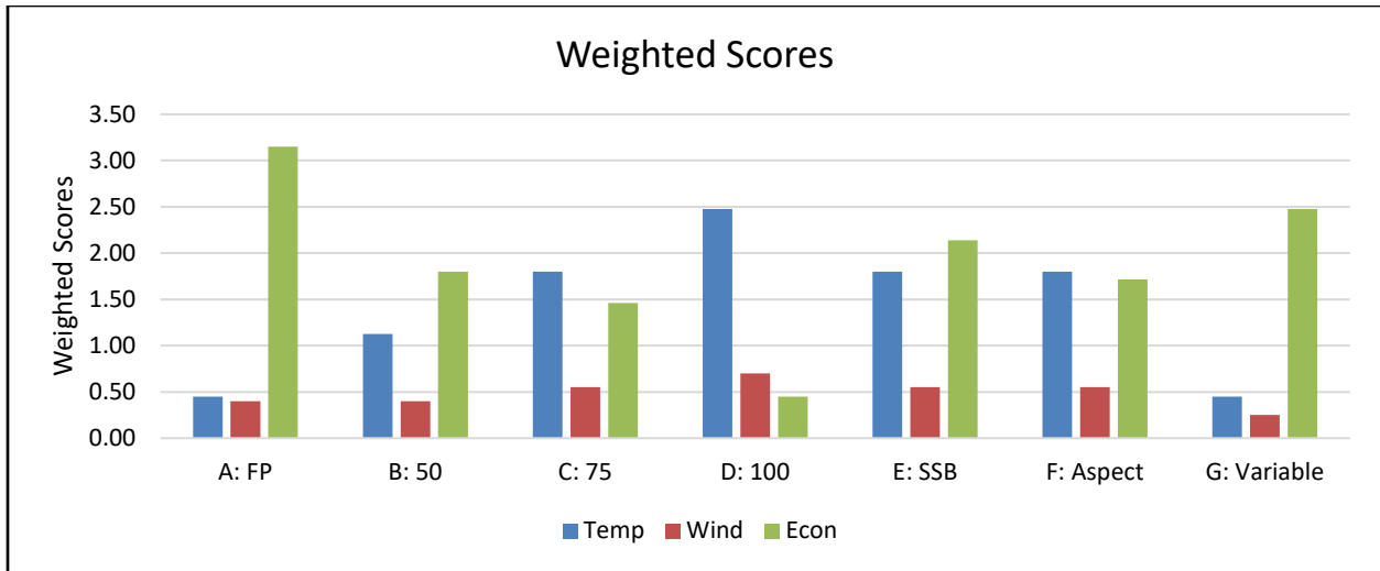
Figure A5: Weighted scores for Alternatives A through G, unstacked. SSB is an acronym for Site-Specific Buffer.
