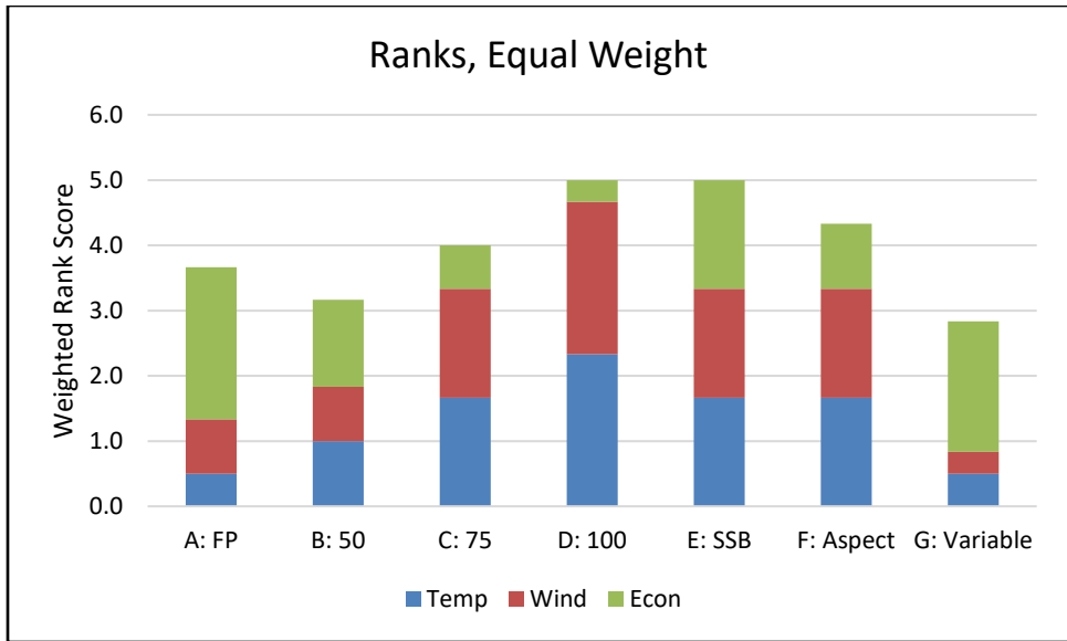
Figure A2. Performance of weighted ranks for Alternatives A through G. SSB is an acronym for Site Specific Buffer.
