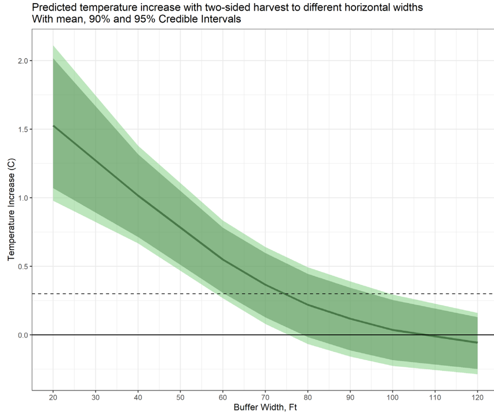
Figure 1: Predicted relationship between two-sided buffer width and stream temperature increase post-harvest. This prediction was based on the data and analysis approach of Groom et al. (2018).
