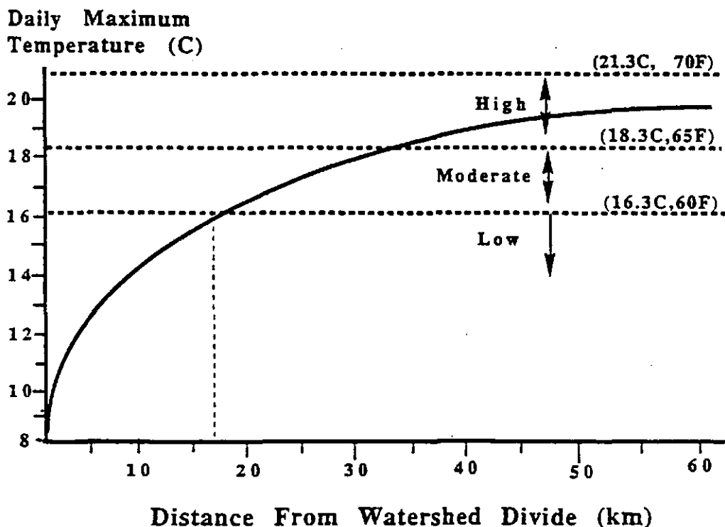
Figure 2.2 Estimated baseline daily maximum temperature during the warmest summer days under a mature forest canopy as a function of distance downstream from watershed divide.
