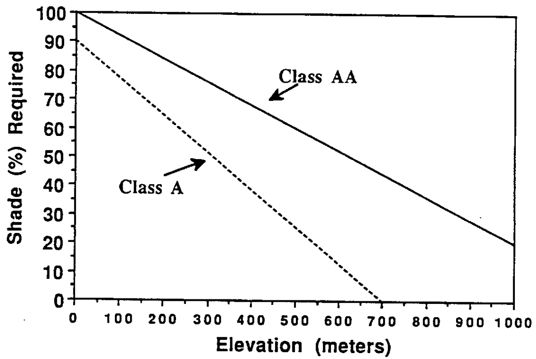
Fig. 6.1 Shade requirements to meet the Washington Water Quality Temperature Criteria (WAC-173-201).
