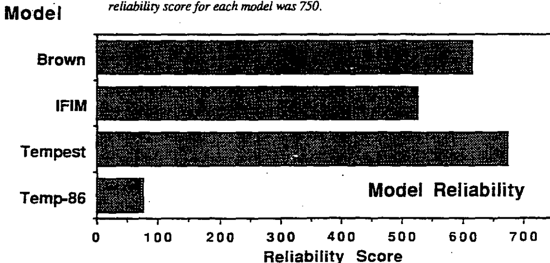
Figure 4.27 Reliability scores for four site models based on model-testing results. Scores are computed based on criteria described in the text. The total possible reliability score for each model was 750.
