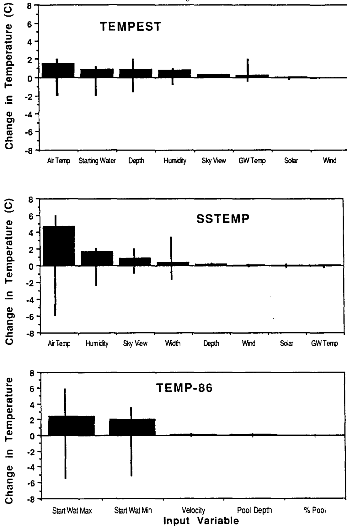
Figure 4.6 Model reliability analysis results showing the range of the predicted mean temperature associated with the observed range of each input variable. Blocks are the 1st standard deviation and bars are the range.
